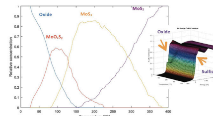
Evolution of XANES spectra and the relative concentration of the four main species as a function of sulfidation temperature.
