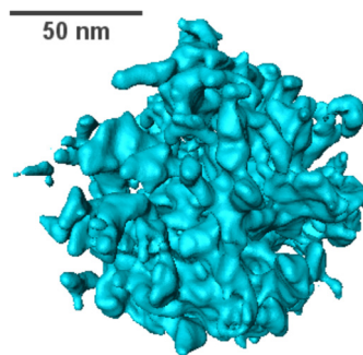
3D visualization of a (reduced) cobalt aggregate obtained by electron tomography.
